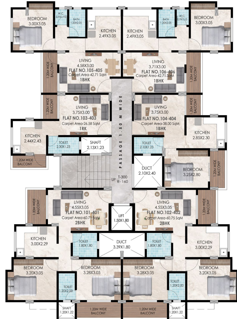
TYPICAL 1st,2nd,3rd & 4th FLOOR PLAN
